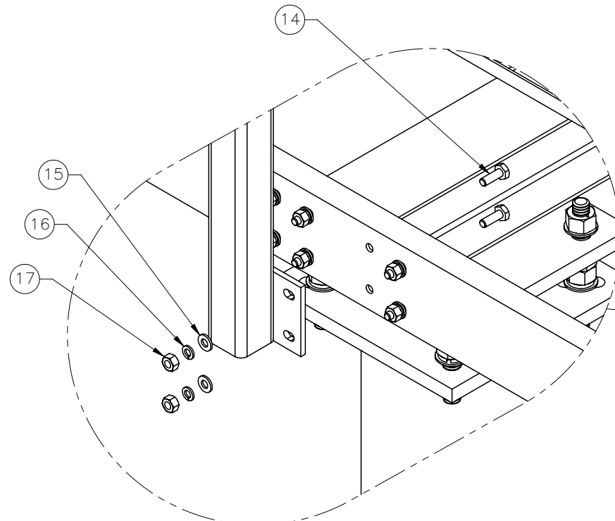
TYPICAL CANOPY CONNECTION
