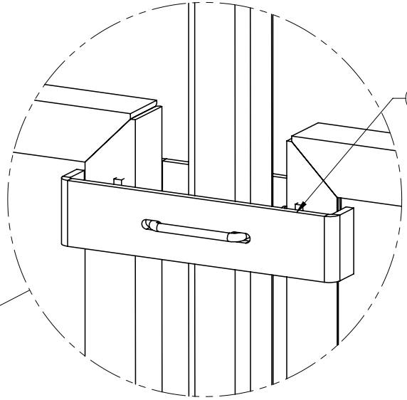
POST BRACKET DETAIL TYP 4X
