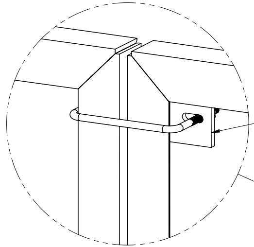
HANDRAIL BRACKET DETAIL 1X
