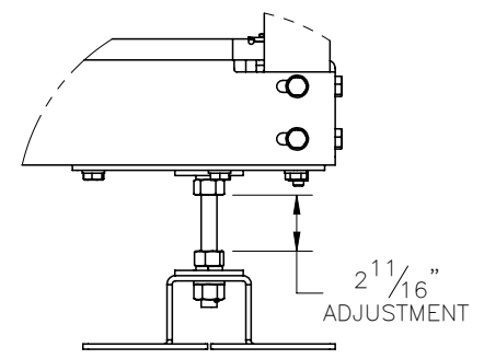
PLATFORM FOOT LEVELING HARDWARE DETAIL B
