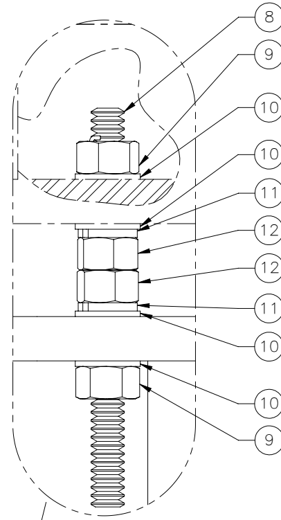
TYP LEVELING HARDWARE DETAIL 4X
