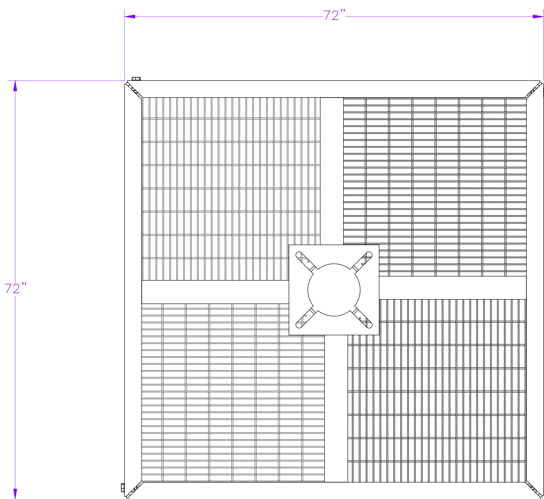
TOP VIEW (SHOWN WITH TOP GRATING REMOVED FOR CLARITY)
