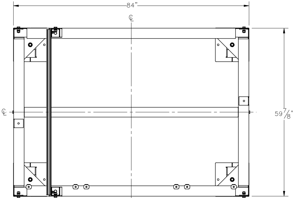
PLAN VIEW (GRATING REMOVED)
