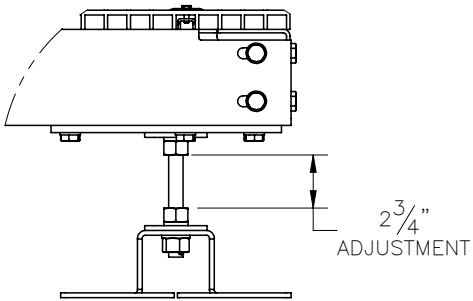
PLATFORM FOOT LEVELING HARDWARE DETAIL B
